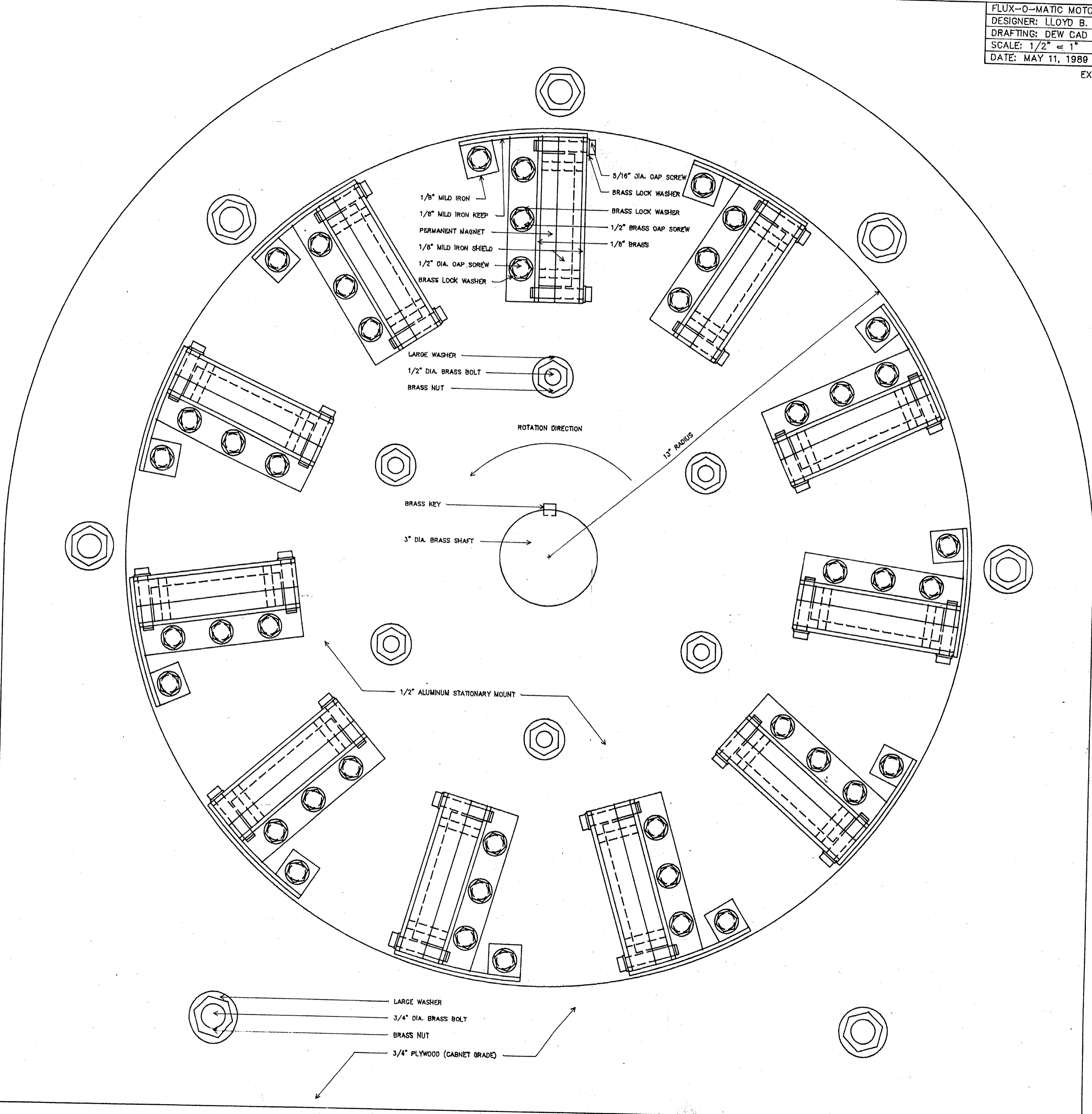
ROTOR MOUNT (LOOKING TOWARDS FRONT)
